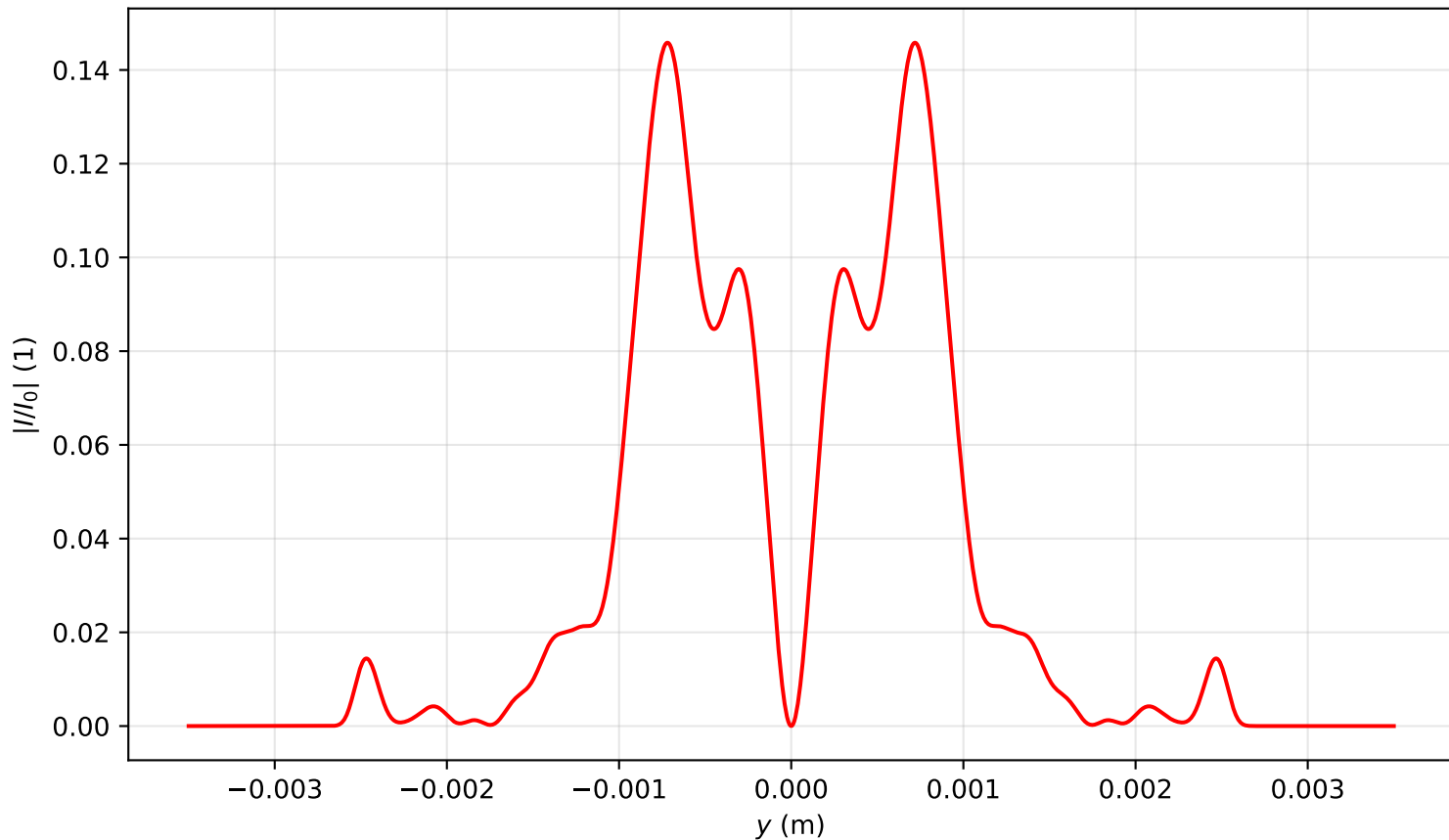
Intensity profile I(x=0, y, z=2.149)/I_0 , P_{in}=8.0P_{cr} , artificial time
